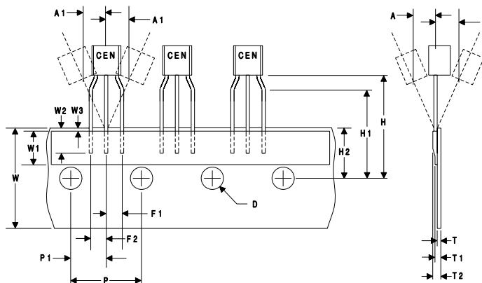
FIGURE 2. TAPING SPECIFICATIONS
